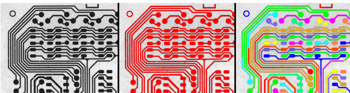
Figure 4.1: Left: Input image of a printed circuit board. Middle: Regions found by threshold , colored red. Right: Connected regions, a result of connection .
